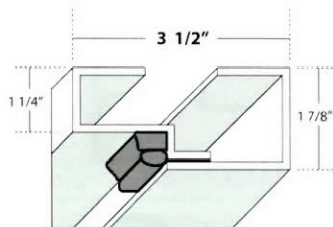
16 GA. STEEL FRAME DUAL CONTACT WEATHER STRIP
